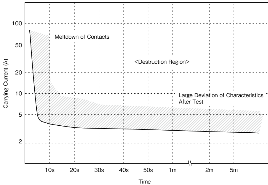
Figure 3.12 Resistance to Carrying Current
