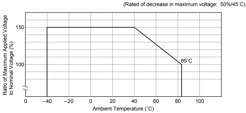
Figure 3.3 Maximum Voltage Applied to Coil
