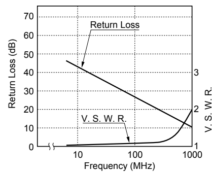
Figure 3.9 High-frequency characteristics
