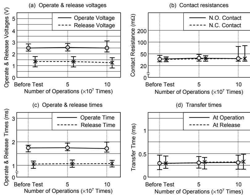
Figure 5.9 Non-load Test A
