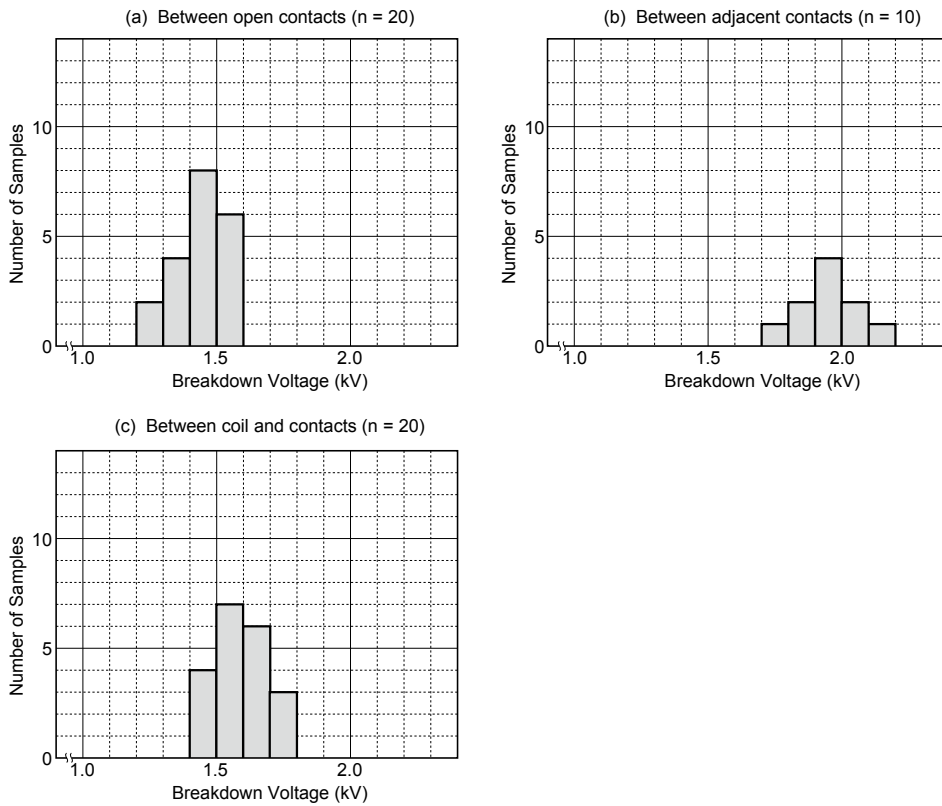
Figure 4.6 Breakdown Voltage
