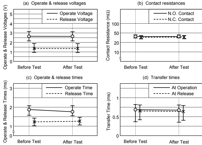
Figure 5.3 (1) Moisture Resistance Test
