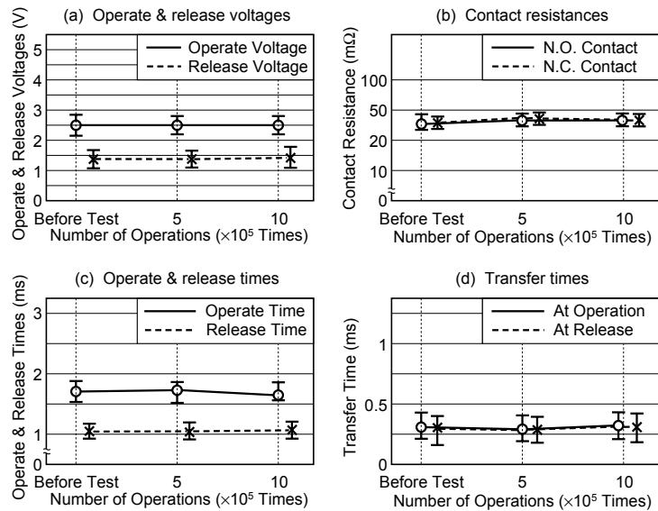
Figure 5.16 Inductive Load Test
