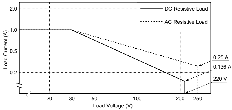
Figure 3.1 Switching Power
