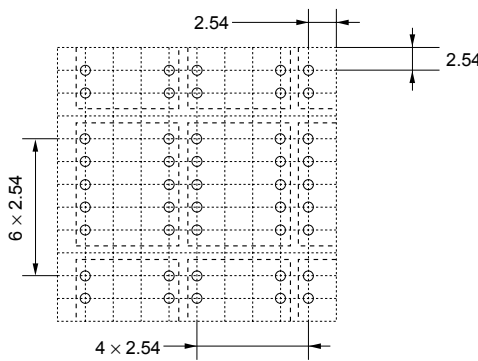
(1) Mounting pitch (mm)
