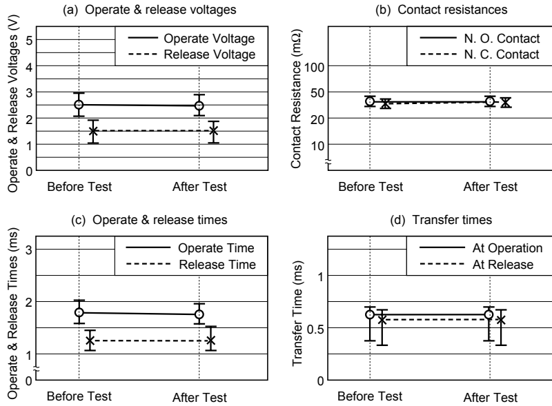
Figure 5.8 (1) Terminal Strength
