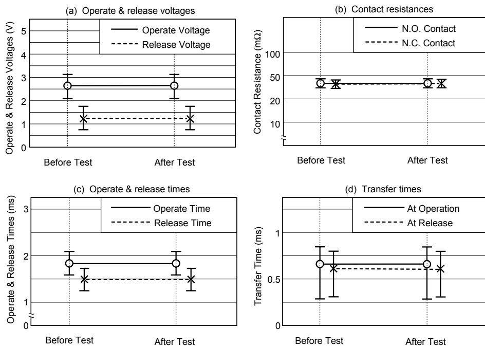
Figure 5.1 (1) High-temperature Test
