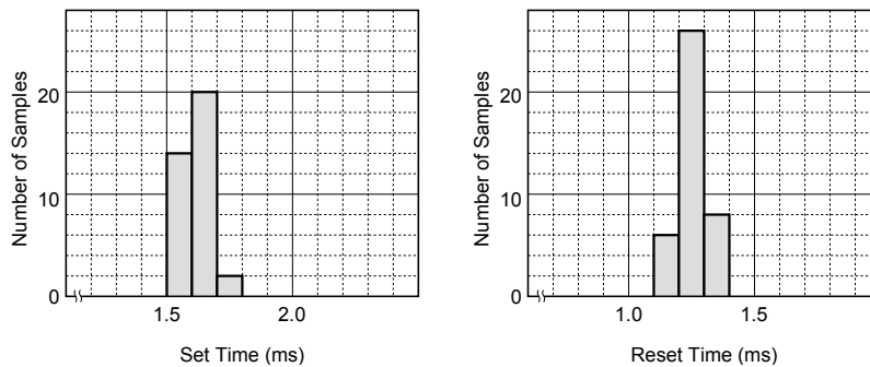
Figure 4.2 Operate & Release Times
