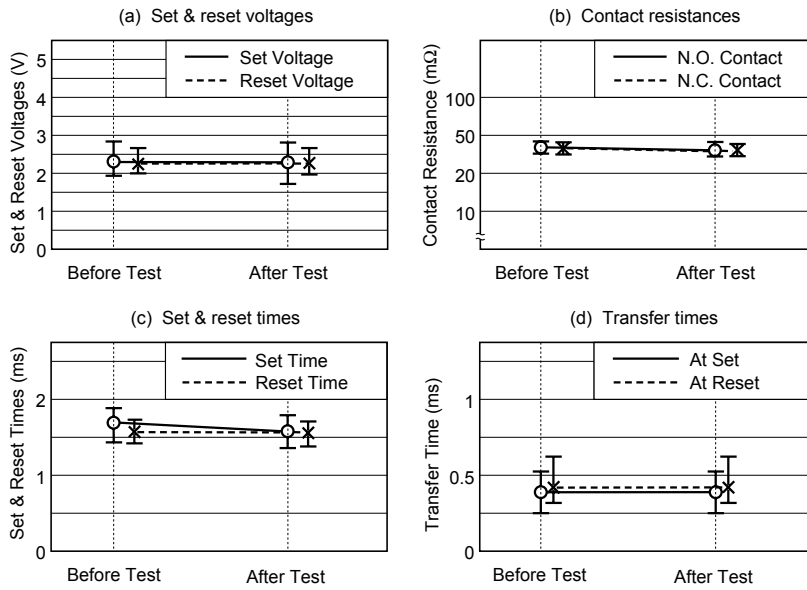
Figure 5.4 (2) Heat Shock Test
