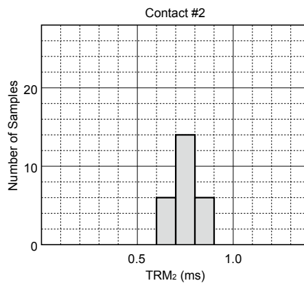
Figure 4.4B Timing
