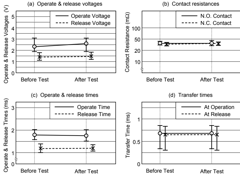
Figure 5.5 (1) Vibration Test
