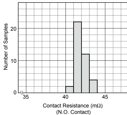
Figure 4.5 Contact Resistance
