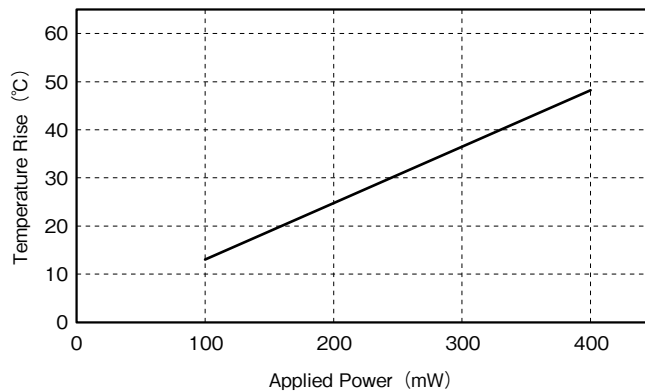
Figure 3.4 Coil Temperature Rise
