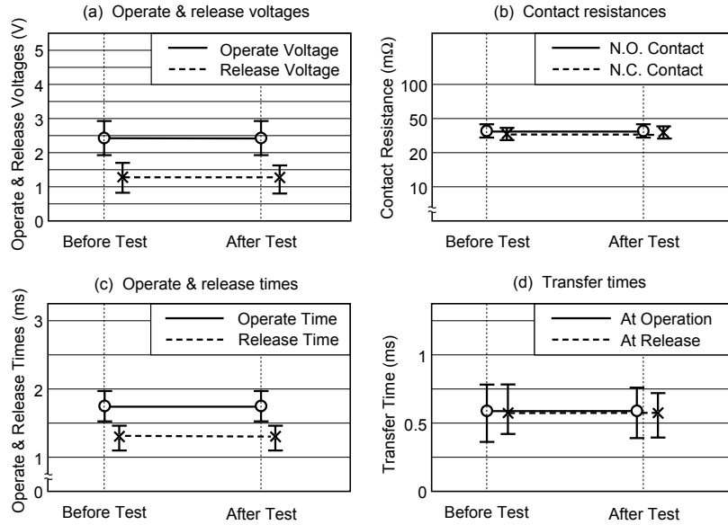
Figure 5.7 (1) Resistance to Solder Heat Test
