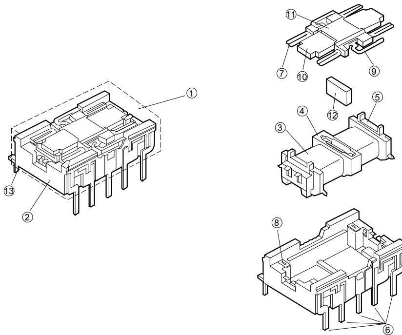
Figure 2.1 Structure of the EA2 Series Relay
