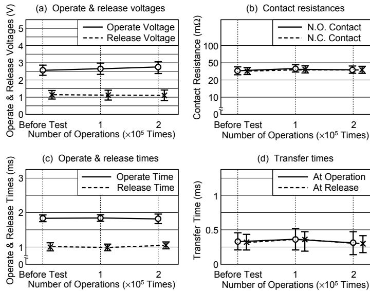
Figure 5.19 Resistive Load Test H
