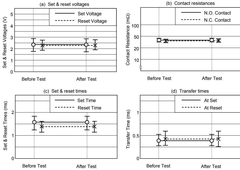
Figure 5.1 (2) High-temperature Test
