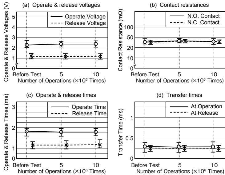
Figure 5.10 Non-load Test B
