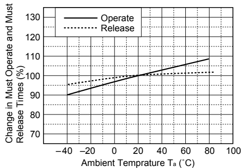
Figure 3.7 Temperature Characteristics
