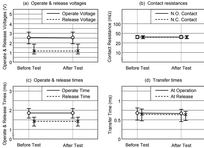
Figure 5.2 (1) Low-temperature Test
