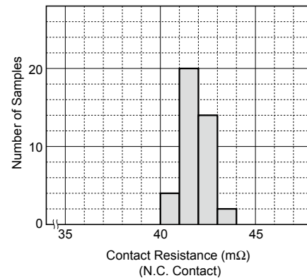
Figure 4.5 Contact Resistance
