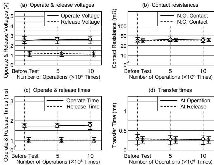
Figure 5.11 Resistive Load Test A
