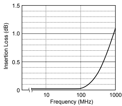
Figure 3.9 High-frequency characteristics
