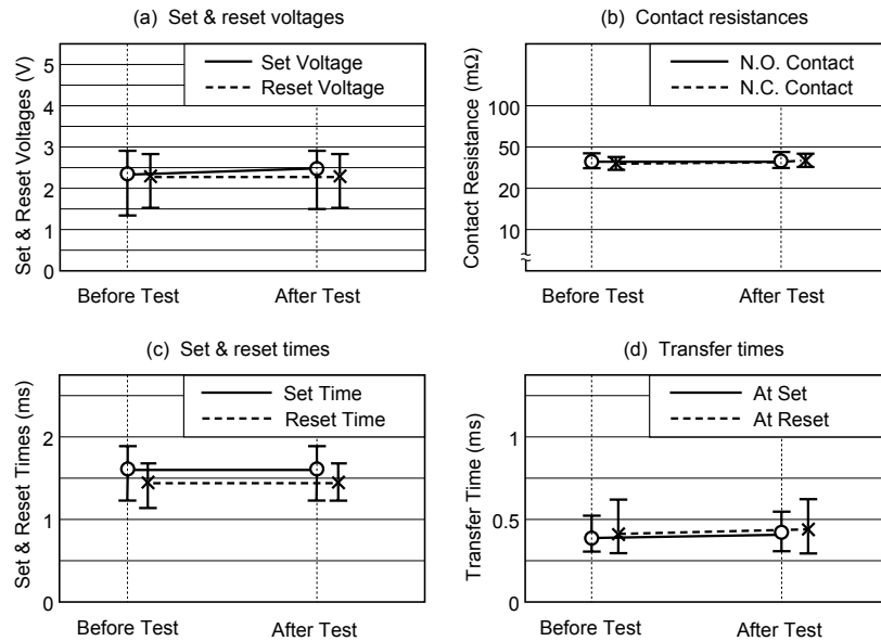
Figure 5.3 (2) Moisture Resistance Test
