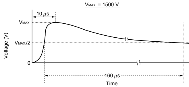
Figure 3.10 Surge Voltage Waveform
