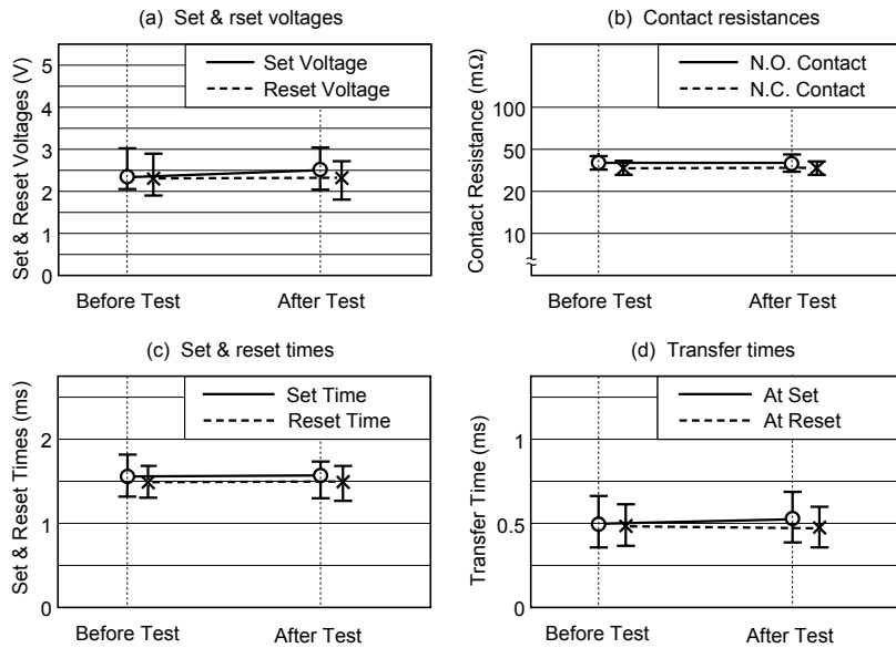
Figure 5.5 (2) Vibration Test
