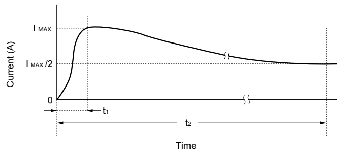
Figure 3.11 Surge Current Waveform
