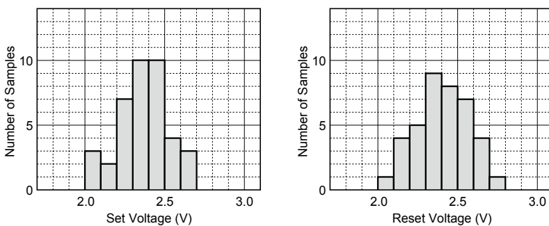
Figure 4.1 Operate & Release Voltages
