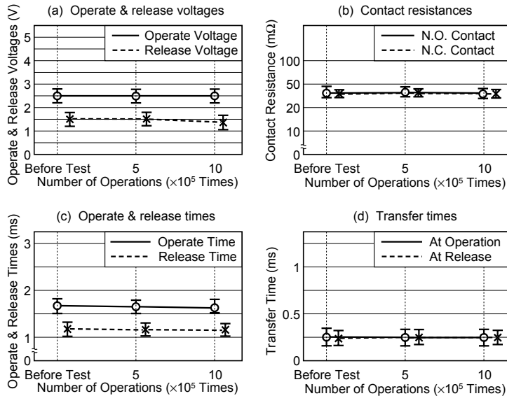
Figure 5.15 Resistive Load Test E
