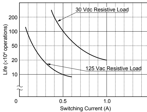
Figure 3.2 Life Curve
