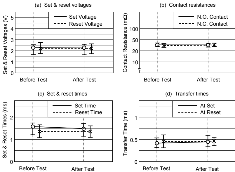
Figure 5.6 (2) Shock Test
