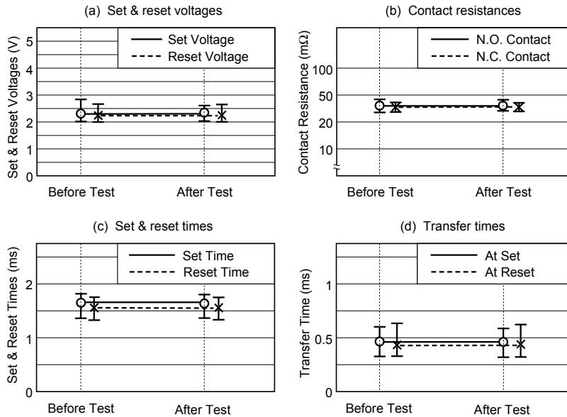
Figure 5.8 (2) Terminal Strength
