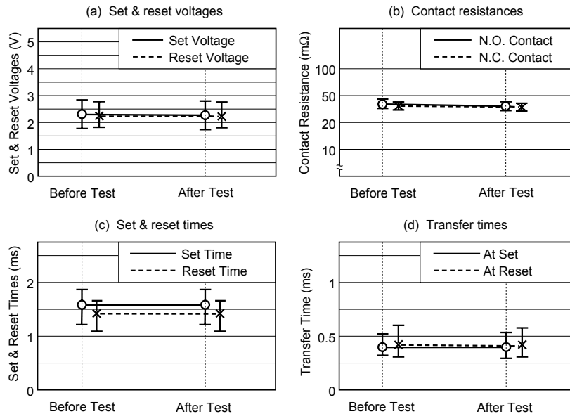
Figure 5.2 (2) Low-temperature Test
