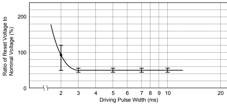
Figure 3.6 Driving Pulse Width vs. Set & Reset Voltages
