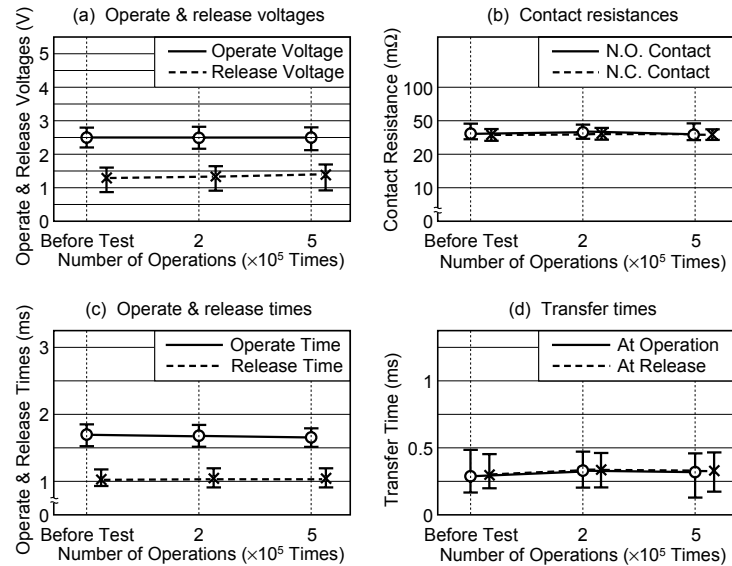
Figure 5.13 Resistive Load Test C
