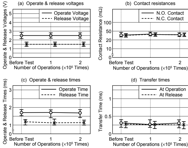
Figure 5.18 Resistive Load Test G
