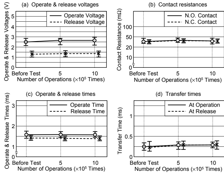
Figure 5.12 Resistive Load Test B
