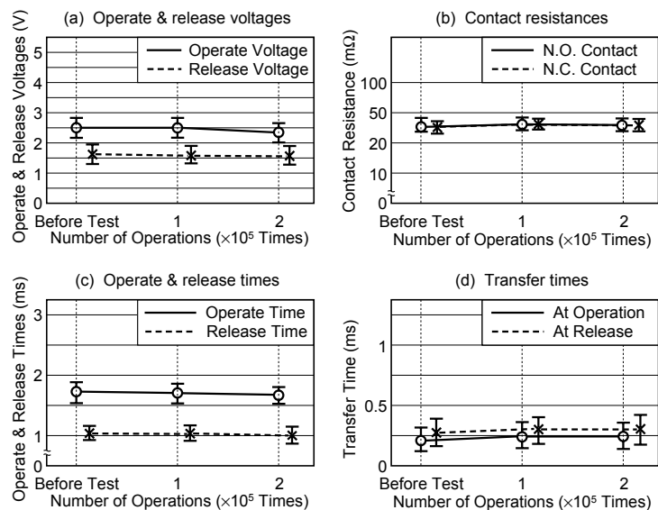
Figure 5.17 Resistive Load Test F
