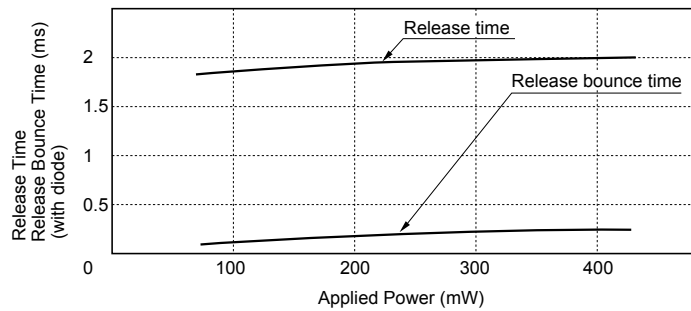
Figure 3.5 Driving Power vs. Timing
