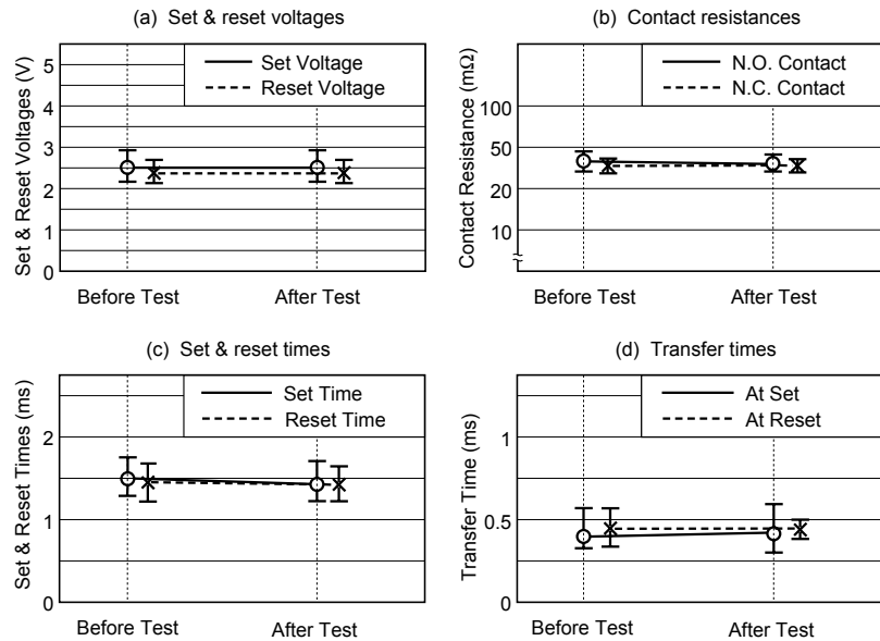
Figure 5.7 (2) Resistance to Solder Heat Test
