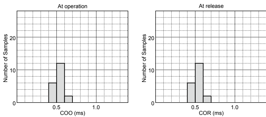
Figure 4.4D Timing
