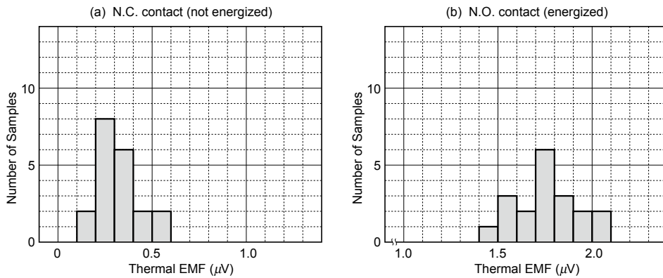
Figure 4.7 Thermal EMF
