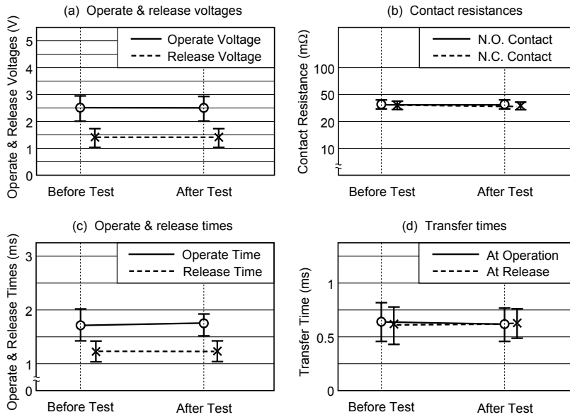
Figure 5.6 (1) Shock Test
