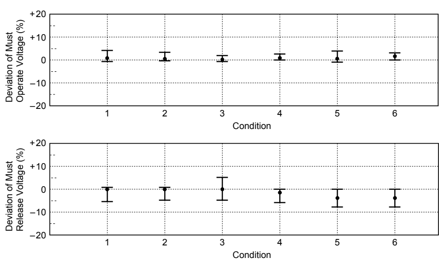
Figure 3.8 Magnetic Interference
