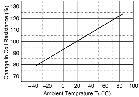
Figure 3.7 Temperature Characteristics
