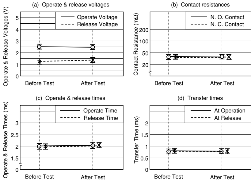
Figure 5.9 (1) Terminal Strength
