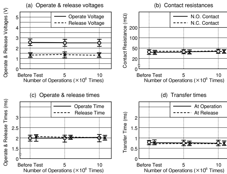
Figure 5.12 Resistive Load Test A
