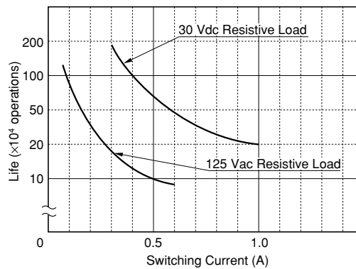
Figure 3.2 Life Curve
