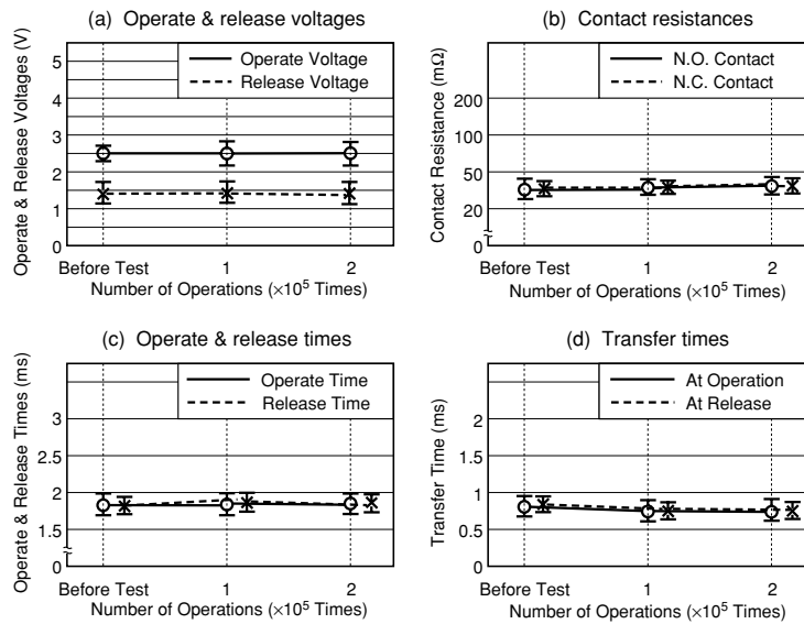
Figure 5.18 Resistive Load Test F
