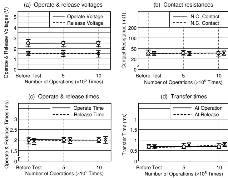
Figure 5.13 Resistive Load Test B
