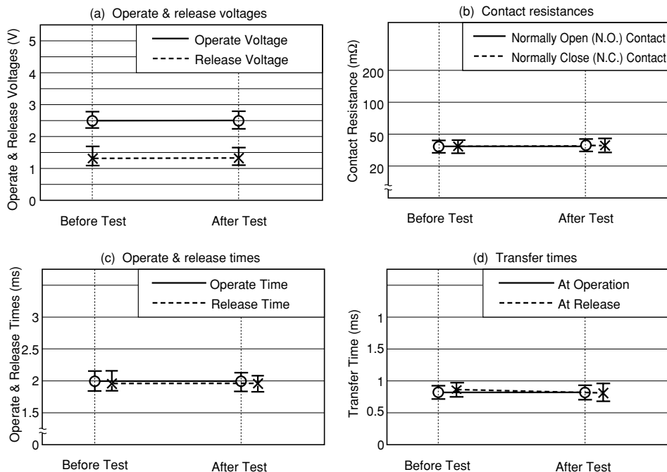
Figure 5.1 (1) High-temperature Test
