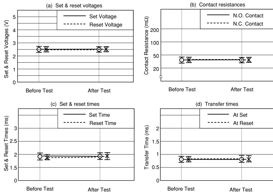
Figure 5.1 (4) High-temperature Test
