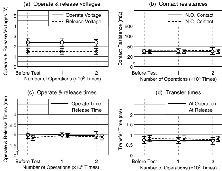
Figure 5.19 Resistive Load Test G
