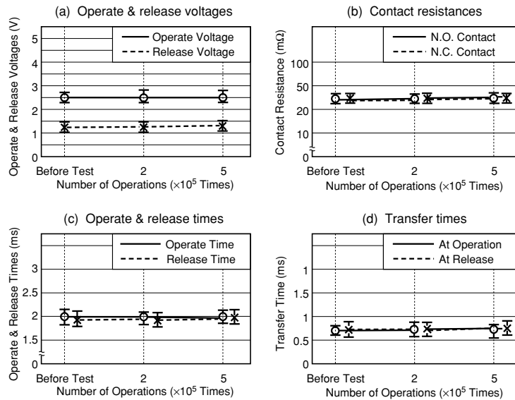
Figure 5.14 Resistive Load Test C
