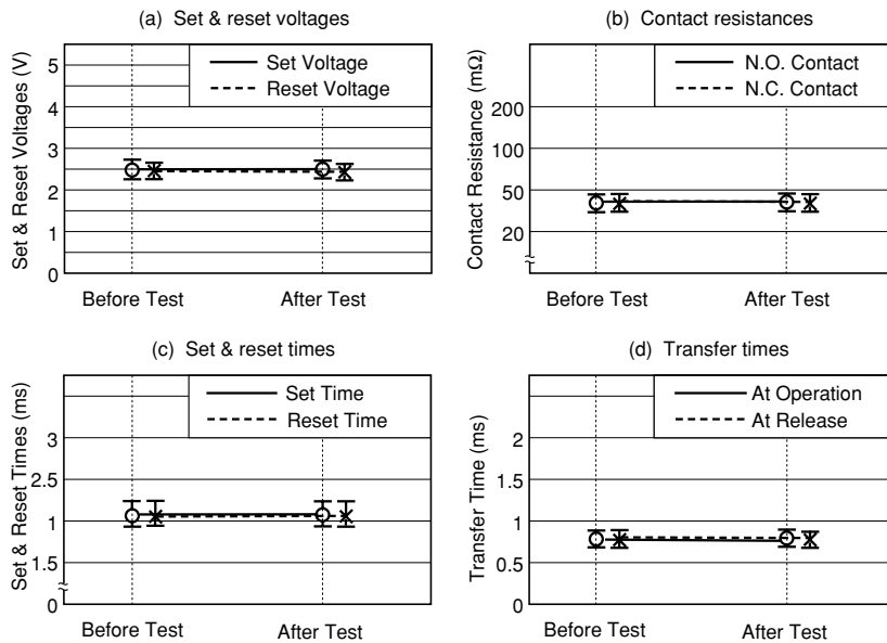
Figure 5.2 (2) Low-temperature Test
