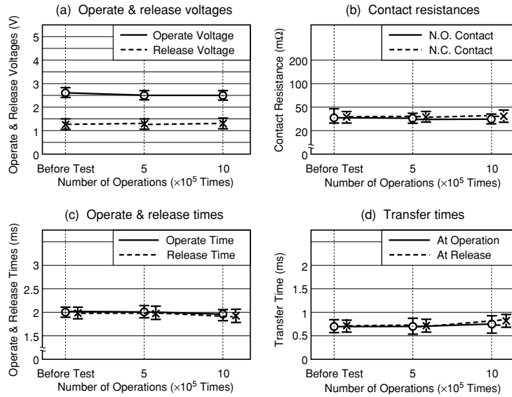
Figure 5.17 Inductive Load Test
