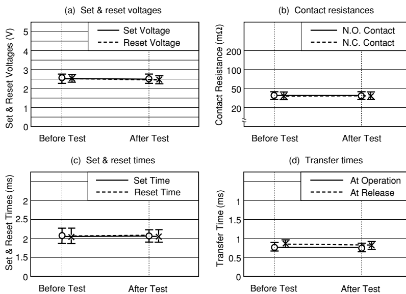
Figure 5.5 (2) Vibration Test
