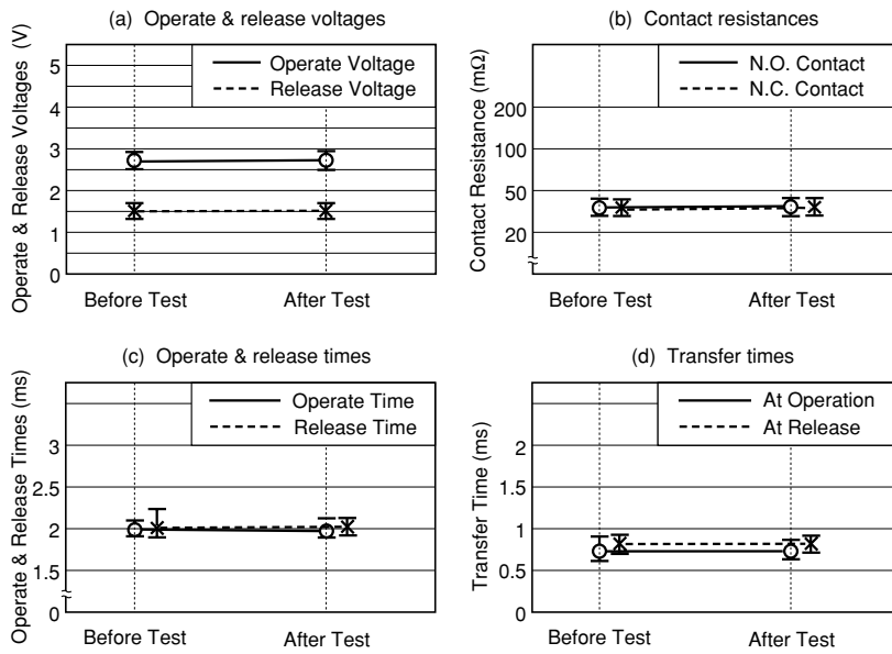
Figure 5.5 (3) Vibration Test
