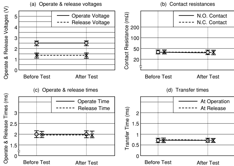
Figure 5.4 (1) Heat Shock Test
