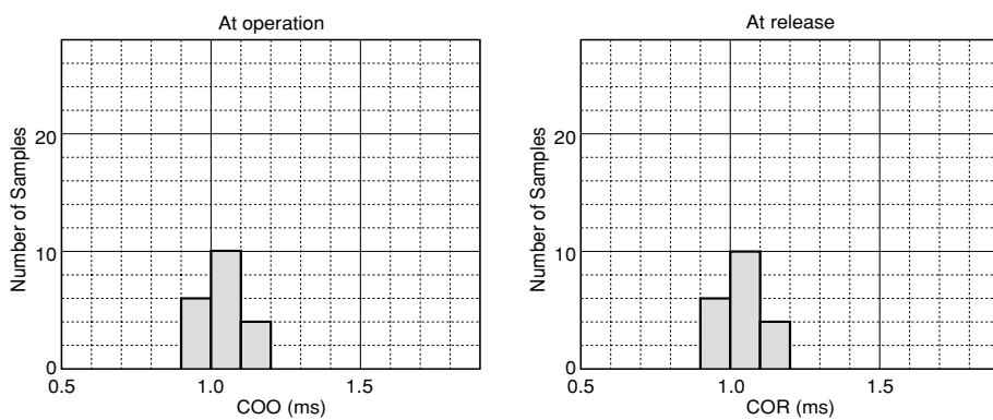
Figure 4.4D Timing
