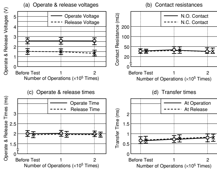
Figure 5.20 Resistive Load Test H
