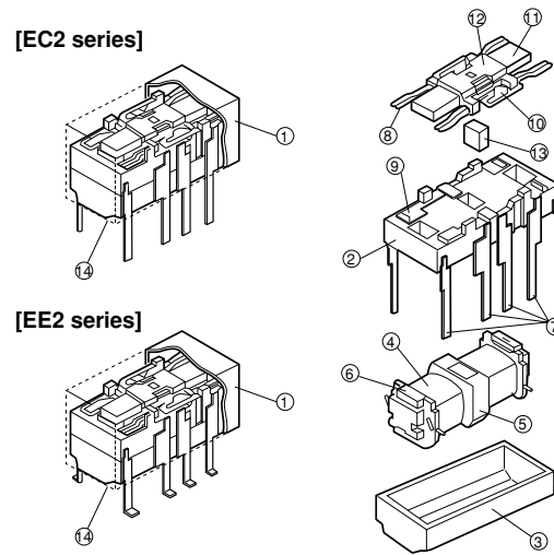
Figure 2.1 Structure of the EC2/EE2 Series Relay
