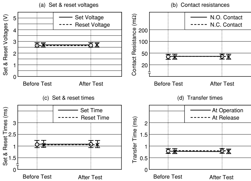
Figure 5.2 (4) Low-temperature Test
