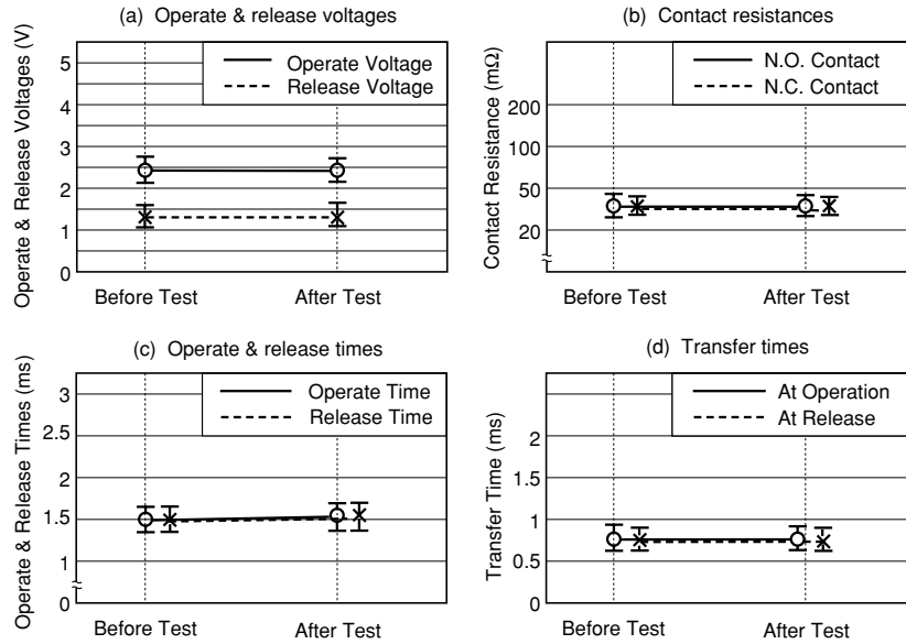
Figure 5.7 (1) Resistance to Solder Heat Test
