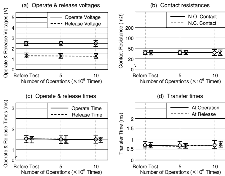
Figure 5.11 Non-load Test B
