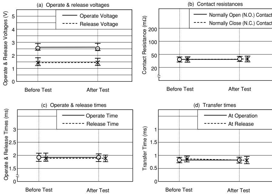
Figure 5.1 (3) High-temperature Test
