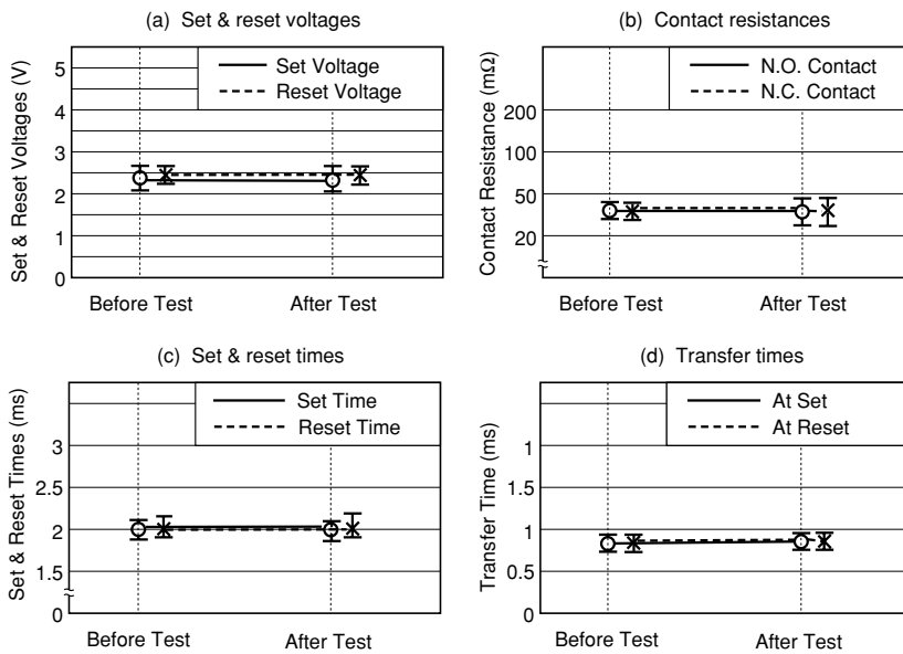
Figure 5.6 (4) Shock Test
