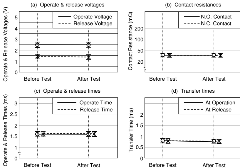
Figure 5.3 (1) Moisture Resistance Test
