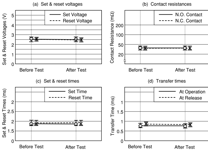
Figure 5.5 (4) Vibration Test
