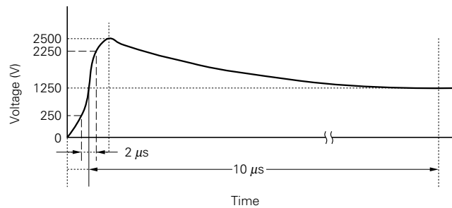
Figure 3.11 Surge Current Waveform
