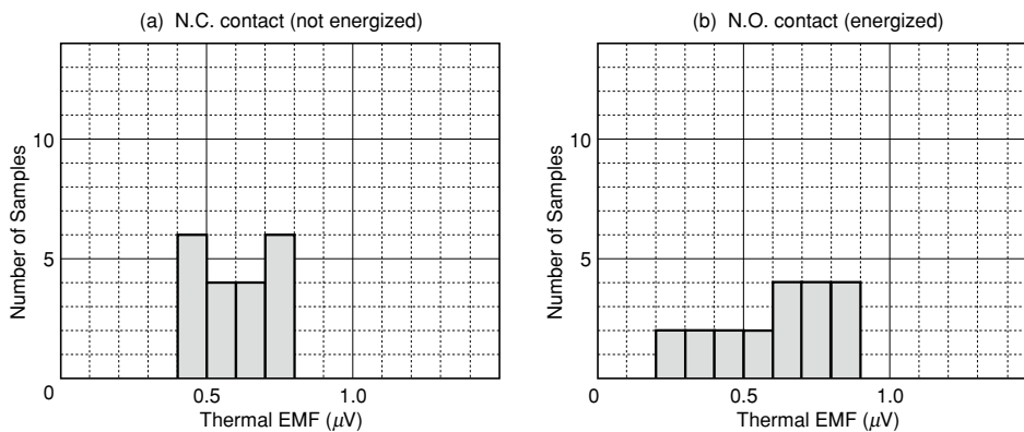
Figure 4.7 Thermal EMF
