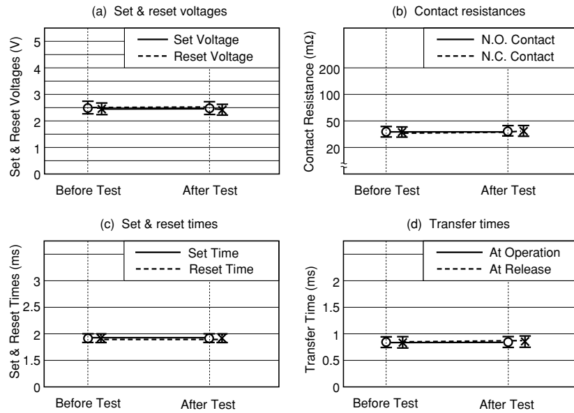
Figure 5.3 (4) Moisture Resistance Test
