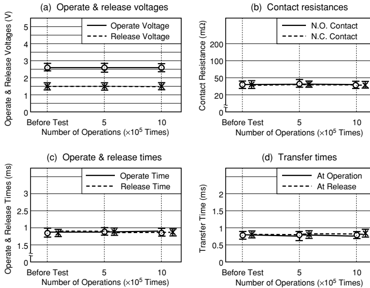
Figure 5.16 Resistive Load Test E
