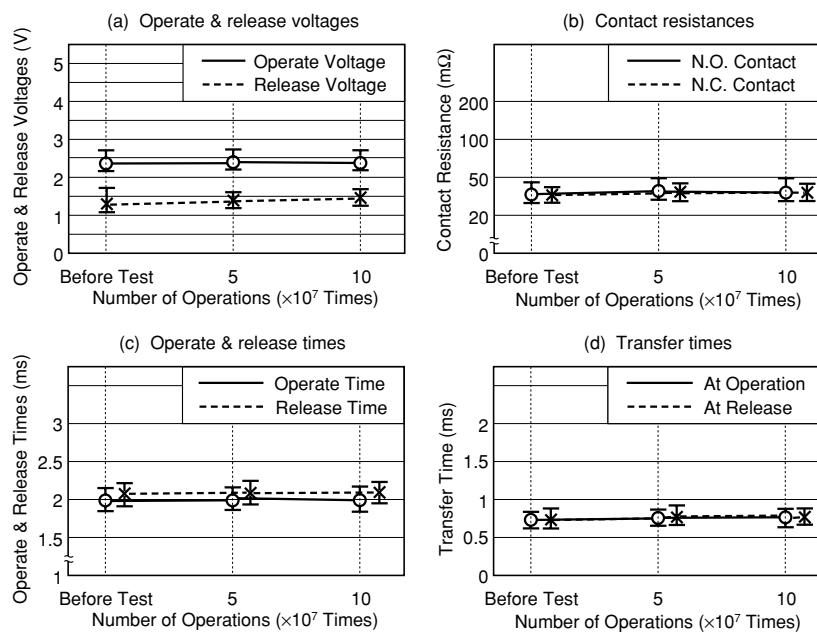
Figure 5.10 Non-load Test A
