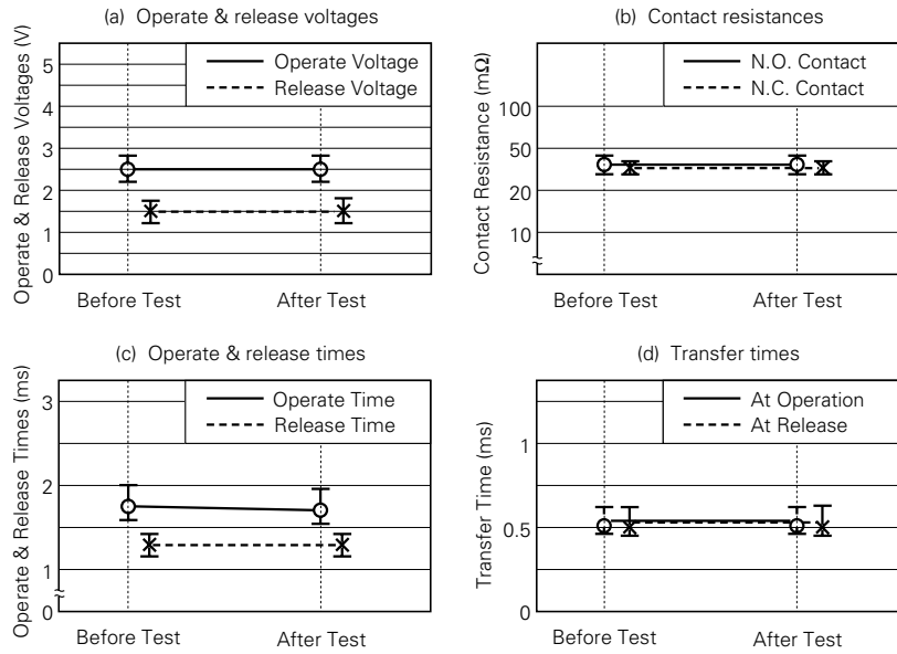
Figure 5.8 (2) Resistance to Reflow Solder Heat
