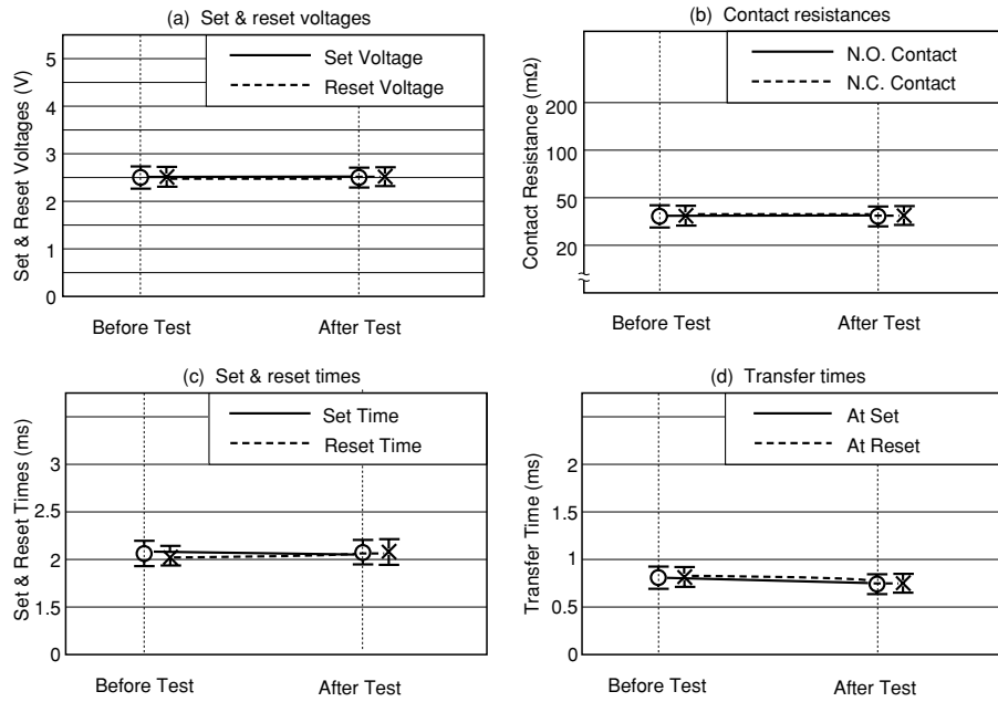
Figure 5.1 (2) High-temperature Test
