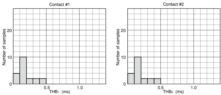
Figure 4.4C Timing
