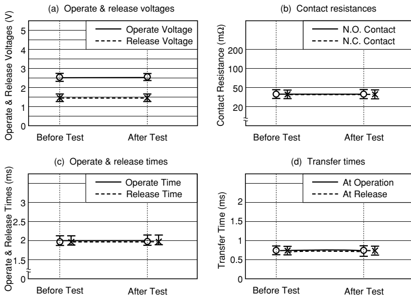
Figure 5.2 (3) Low-temperature Test
