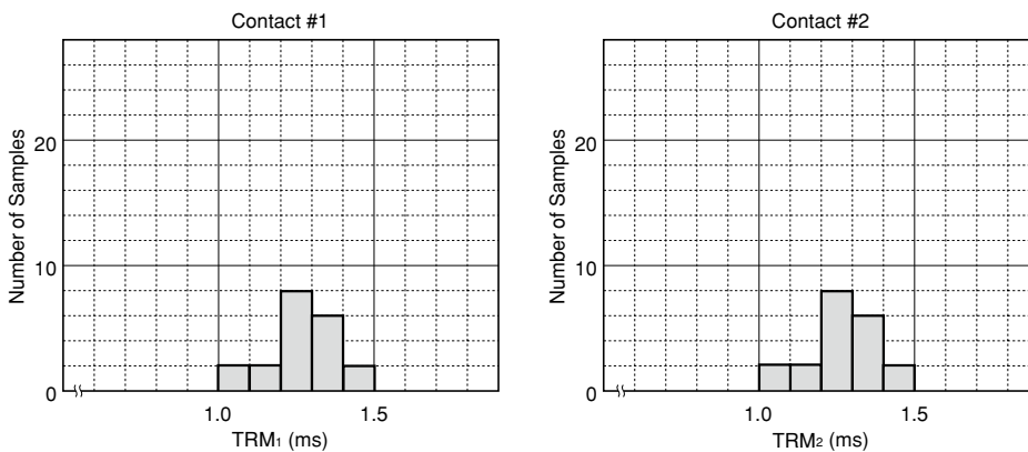
Figure 4.4B Timina
