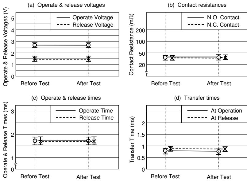
Figure 5.6 (3) Shock Test
