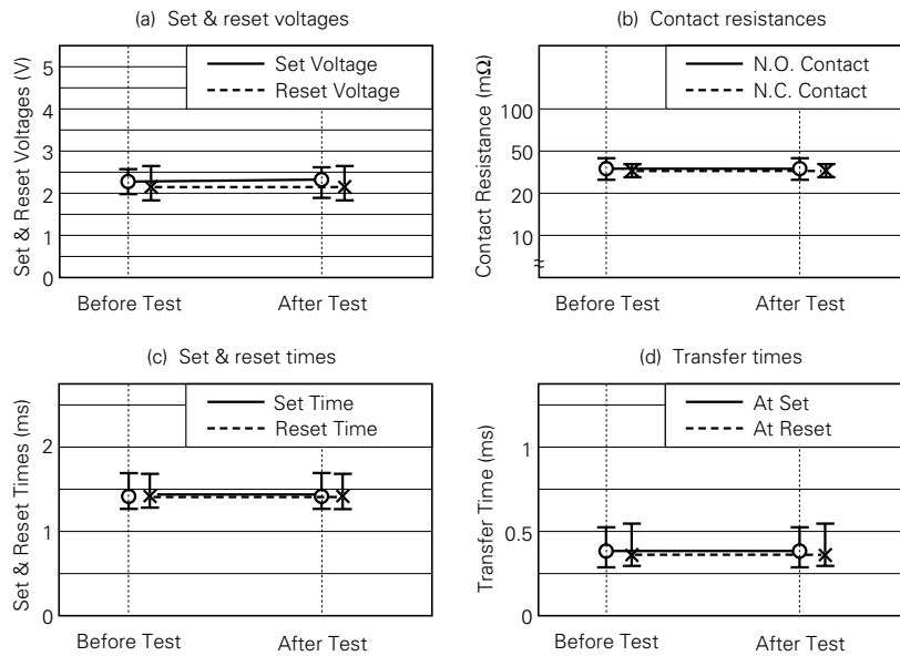
Figure 5.8 (3) Resistance to Reflow Solder Heat
