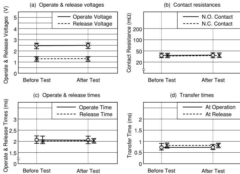
Figure 5.5 (1) Vibration Test
