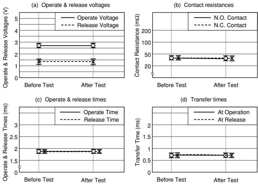
Figure 5.4 (3) Heat Shock Test
