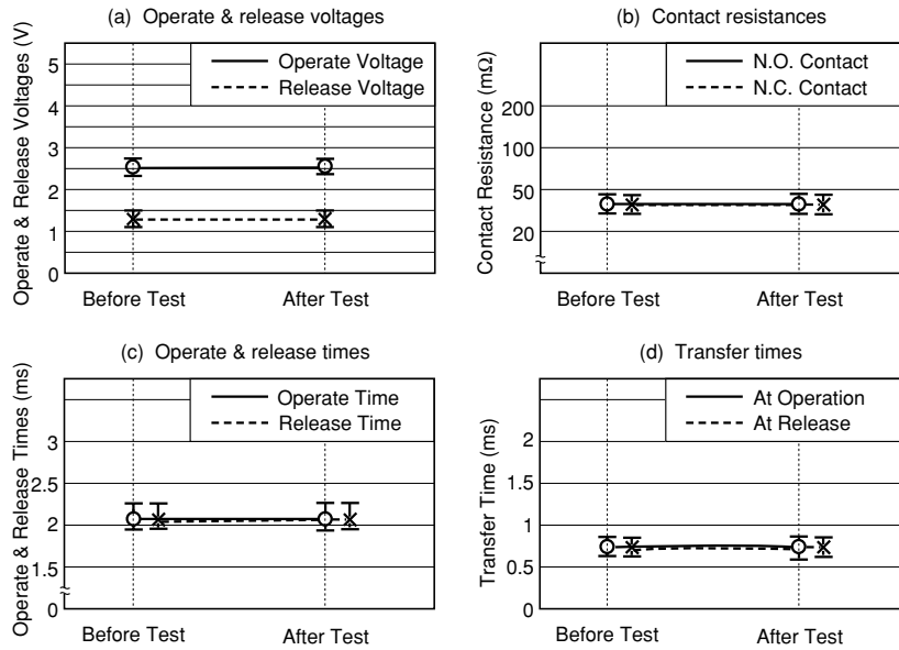
Figure 5.2 (1) Low-temperature Test
