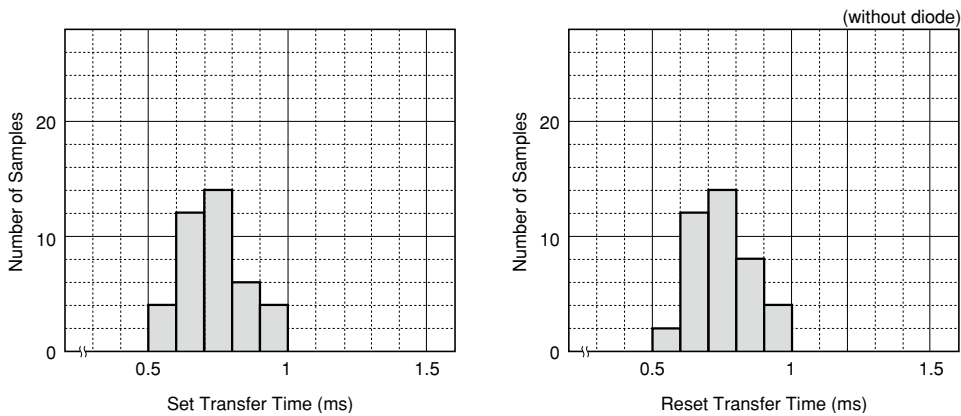
Figure 4.3 Transfer Times
