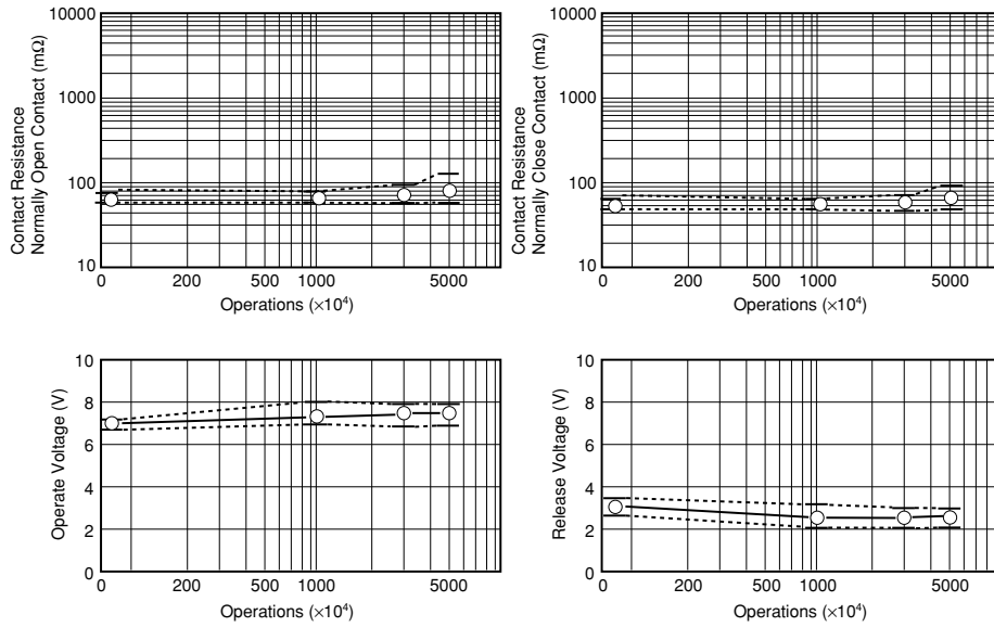
Figure 5.9 (1) Non-load Test A
