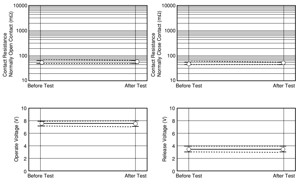
Figure 5.2 (2) Low-temperature Test
