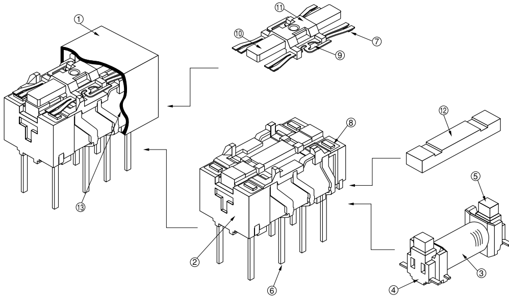
Figure 2.1 Structure of the UA2/UB2 Series Relay
