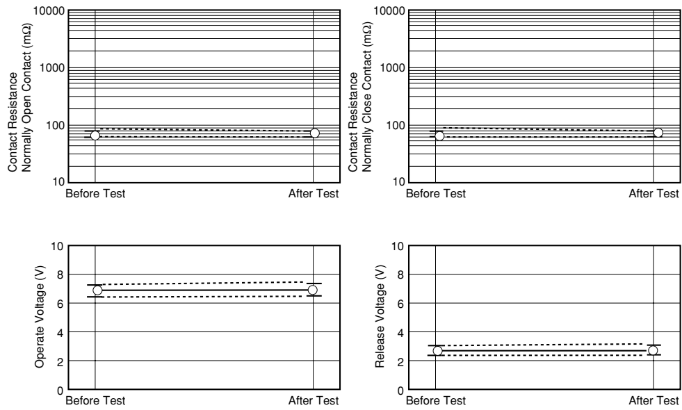
Figure 5.7 Resistance to Solder Heat Test
