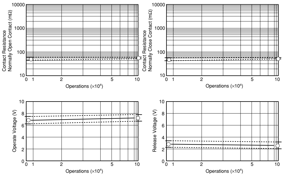
Figure 5.11 (2) Resistive Load Test B
