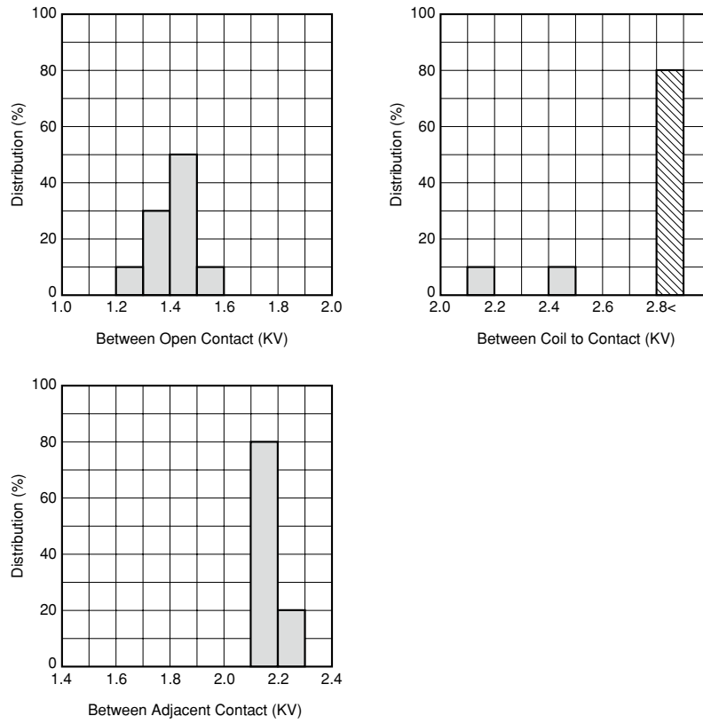
Figure 4.6 Breakdown Voltage
