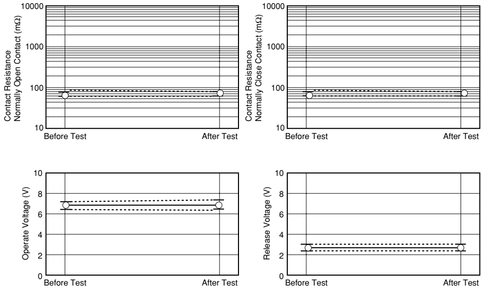
Figure 5.1 (1) High-temperature Test
