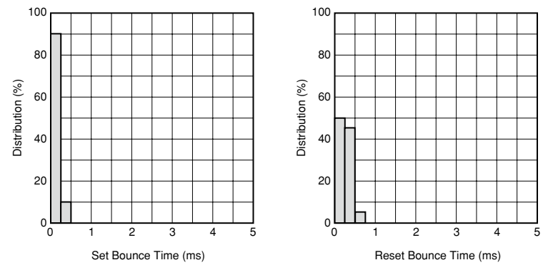
Figure 4.4B Timing
