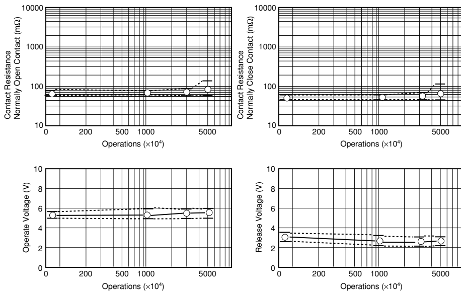
Figure 5.9 (2) Non-load Test A
