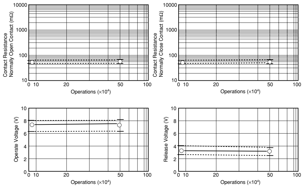
Figure 5.10 (2) Resistive Load Test B
