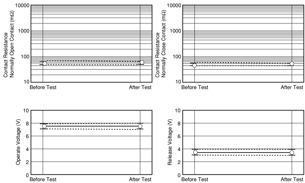
Figure 5.3 (2) Moisture Resistance Test
