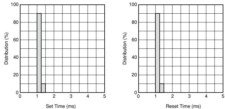
Figure 4.2 Operate & Release Times
