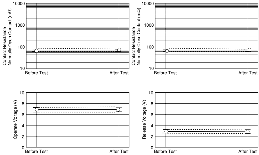
Figure 5.5 (1) Vibration Test
