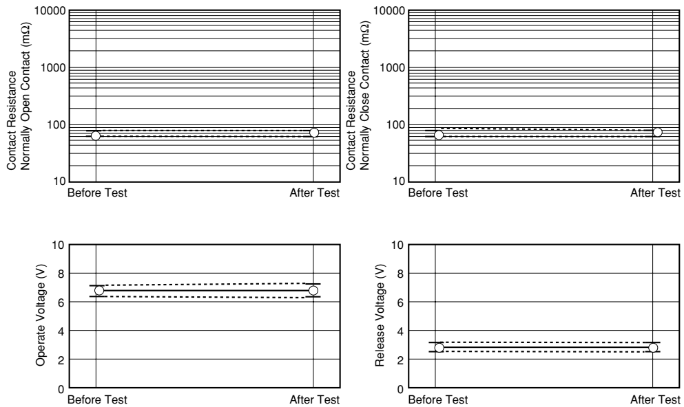
Figure 5.3 (1) Moisture Resistance Test
