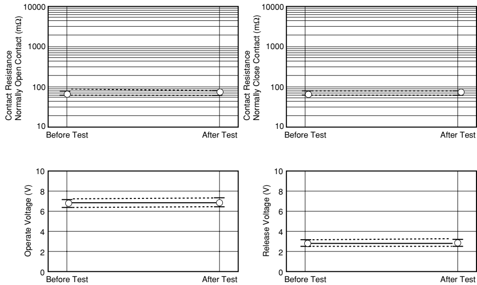
Figure 5.4 (1) Heat Shock Test
