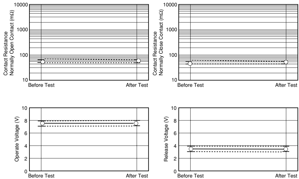
Figure 5.5 (2) Vibration Test
