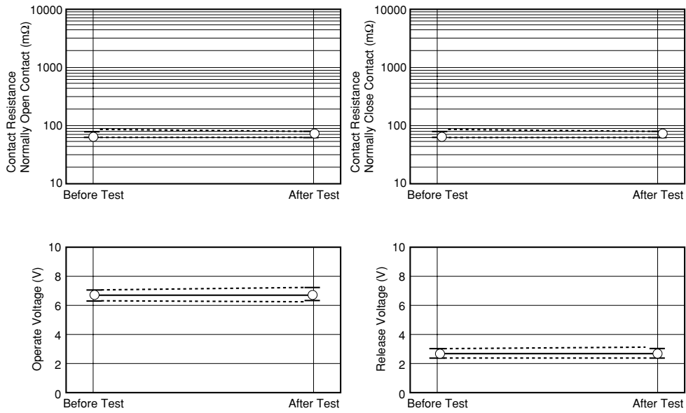
Figure 5.2 (1) Low-temperature Test
