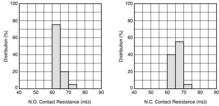
Figure 4.5 Contact Resistance
