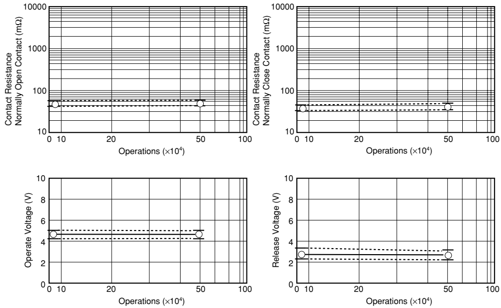
Figure 5.10 (1) Resistive Load Test B
