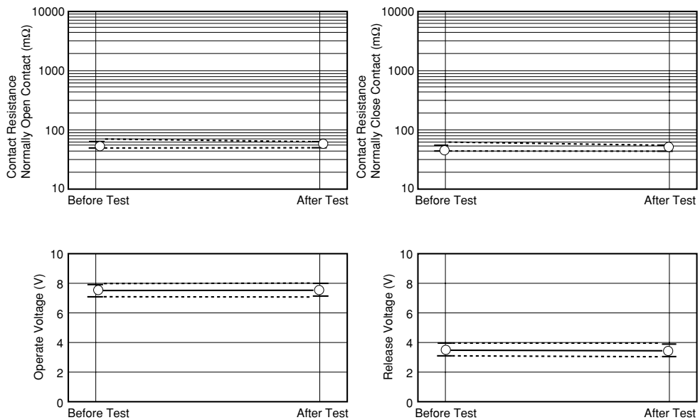
Figure 5.6 (2) Shock Test
