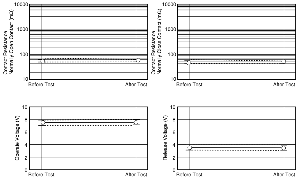
Figure 5.8 Resistance to Reflow Solder Heat
