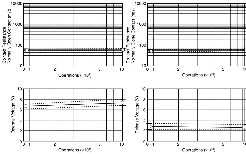
Figure 5.12 (1) Resistive Load Test H
