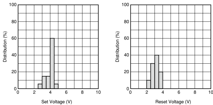
Figure 4.1 Operate & Release Voltages
