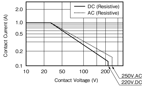
Figure 3.1 Switching Power
