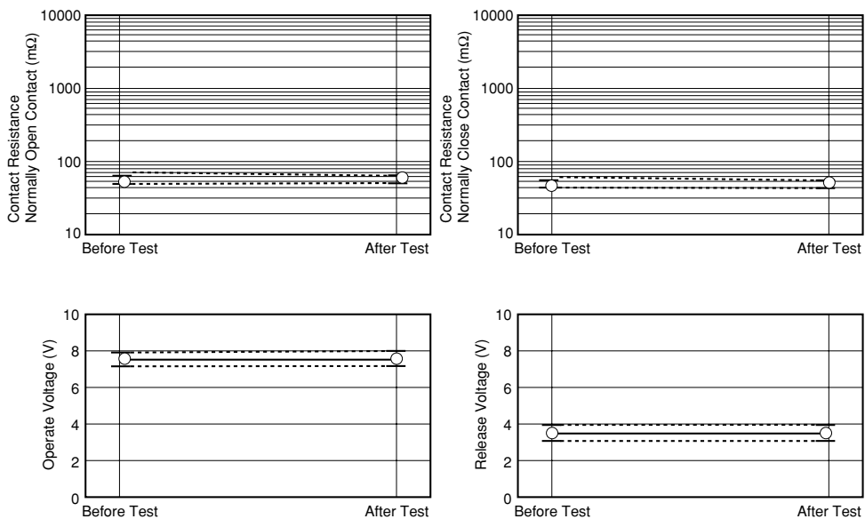
Figure 5.1 (2) High-temperature Test
