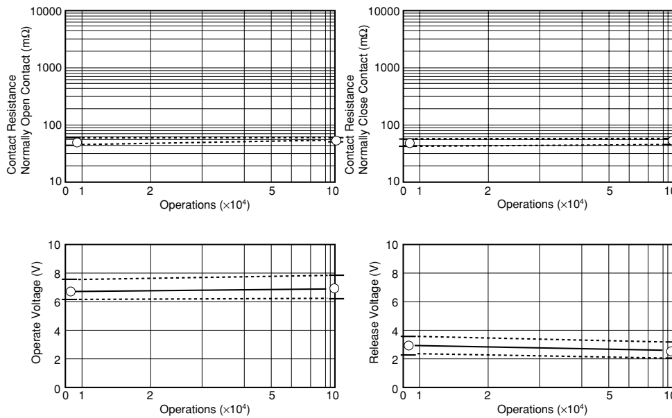
Figure 5.12 (2) Resistive Load Test H
