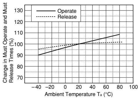
Figure 3.5 Temperature Characteristics
