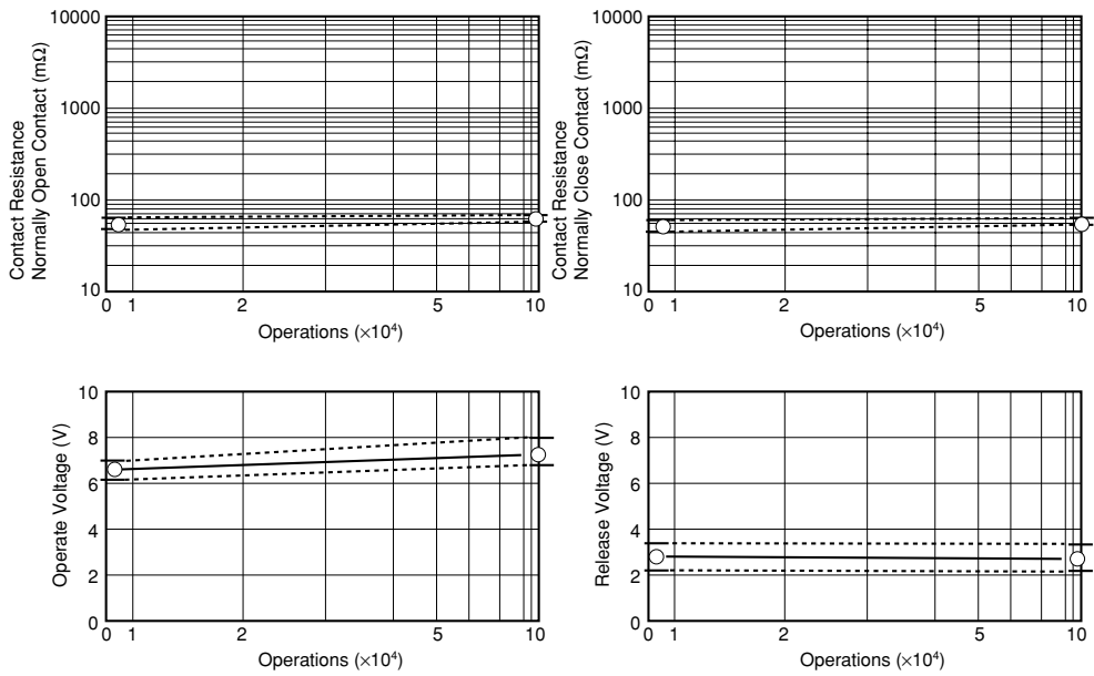
Figure 5.11 (1) Resistive Load Test B
