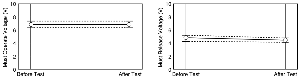
Figure 3.10 Resistance to Carrying Current
