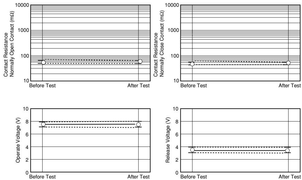
Figure 5.4 (2) Heat Shock Test
