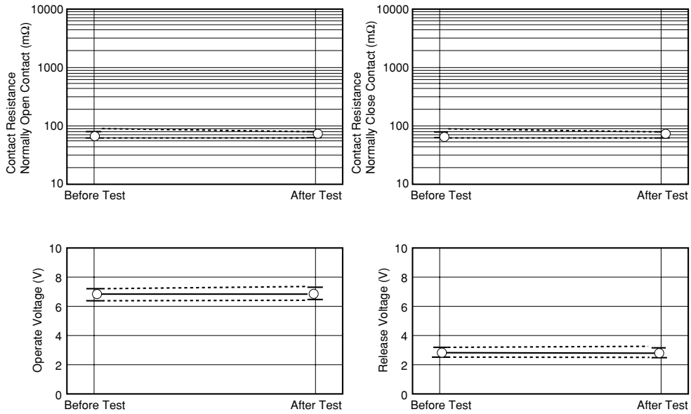
Figure 5.6 (1) Shock Test
