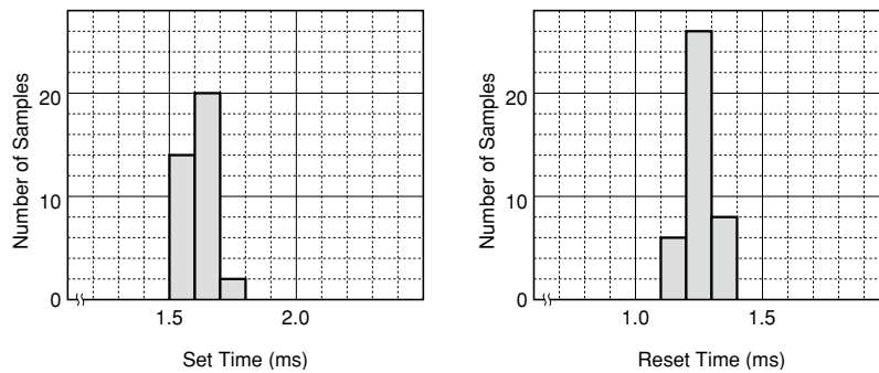
Figure 4.2 Operate & Release Times
