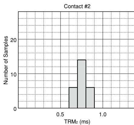
Figure 4.4B Timing
