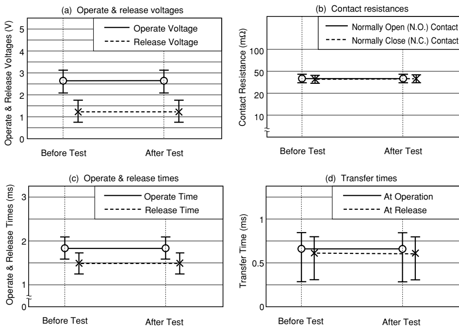
Figure 5.1 (1) High-temperature Test
