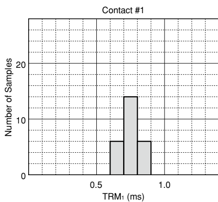
Figure 4.4B Timing
