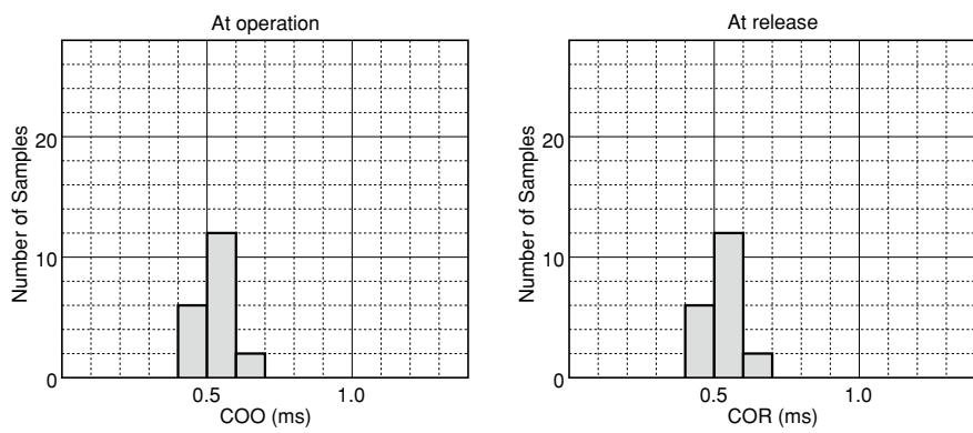
Figure 4.4D Timing
