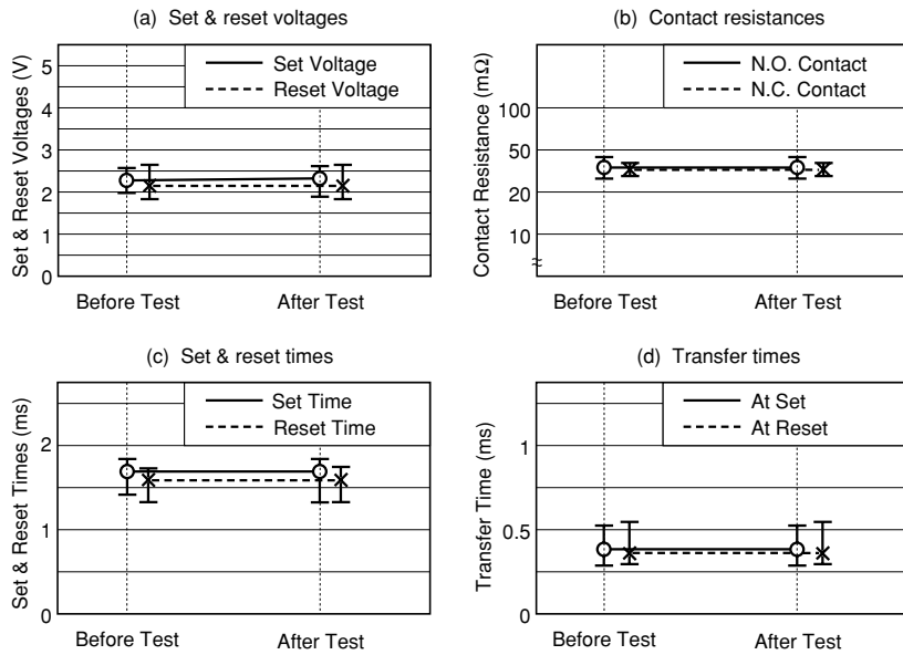
Figure 5.7 (3) Resistance to Reflow Solder Heat
