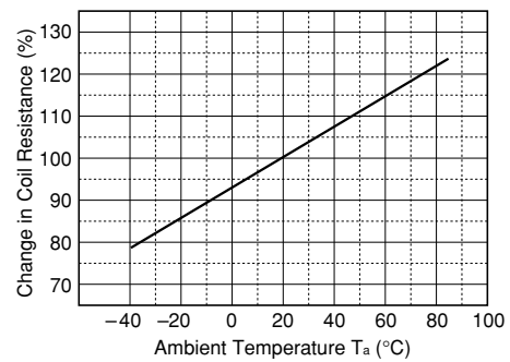
Figure 3.5 Temperature Characteristics
