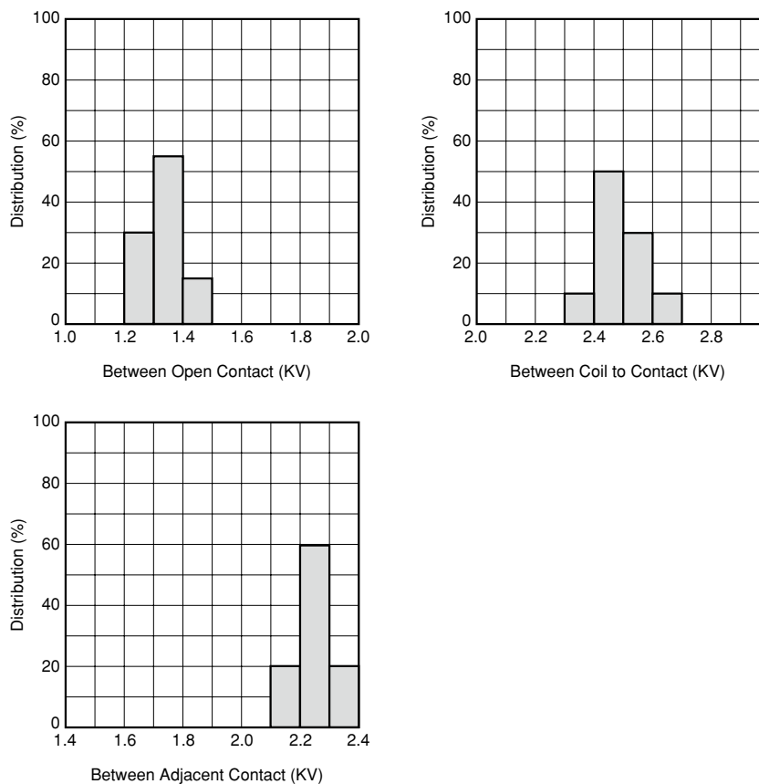
Figure 4.6 Breakdown Voltage
