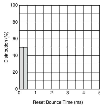
Figure 4.4B Timing
