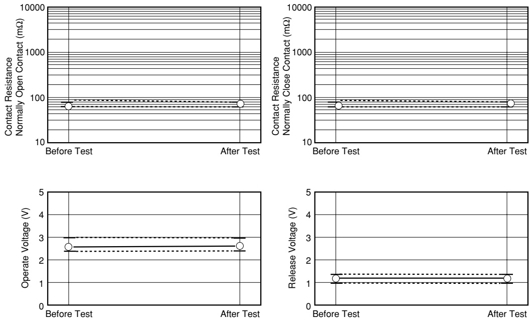
Figure 5.3 (1) Moisture Resistance Test
