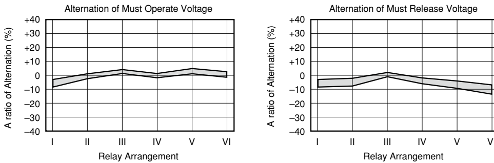
Figure 3.6 Magnetic Interference
