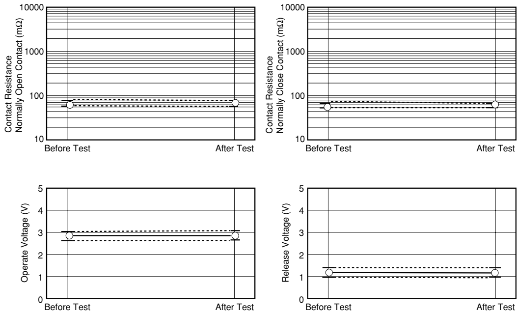
Figure 5.5 (2) Vibration Test
