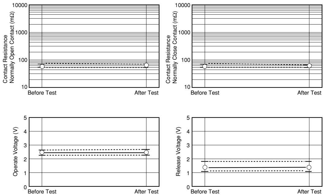
Figure 5.1 (2) High-temperature Test
