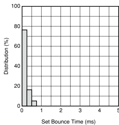
Figure 4.4B Timing
