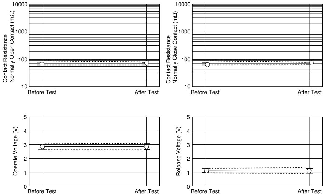
Figure 5.5 (1) Vibration Test
