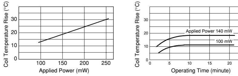
Figure 3.3 Coil Temperature Rise
