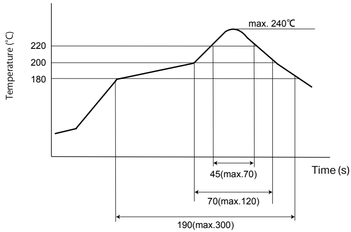
Temperature Profiles
