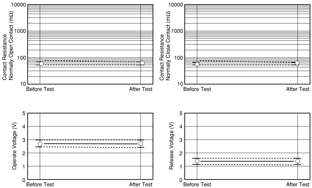
Figure 5.2 (2) Low-temperature Test
