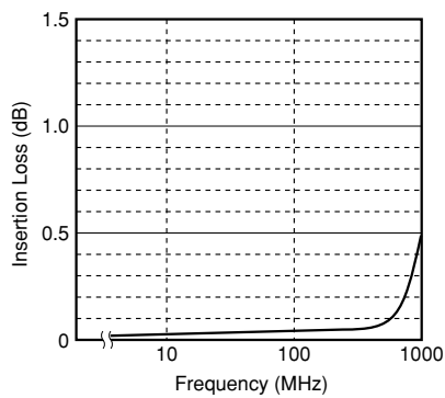
Figure 3.7 High-frequency characteristics
