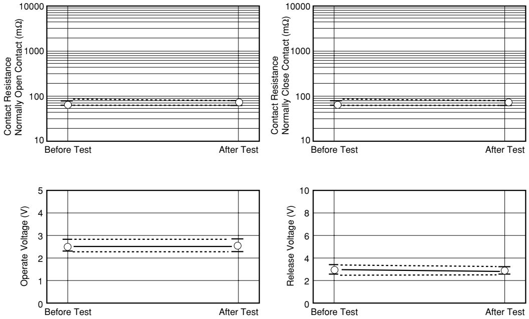
Figure 5.2 (1) Low-temperature Test
