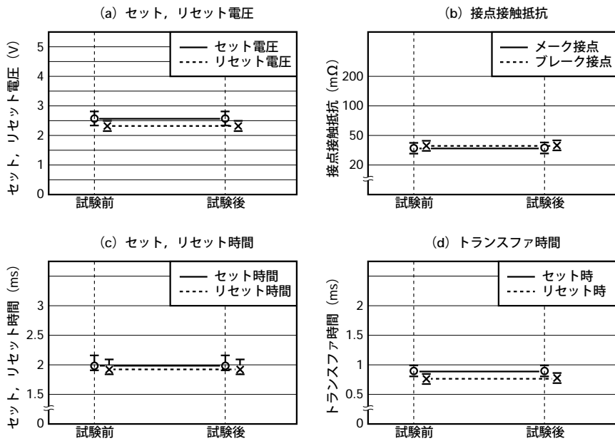
図5.6 (4) 衝撃
