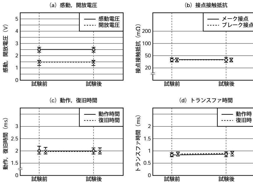
図5.6 (1) 衝撃
