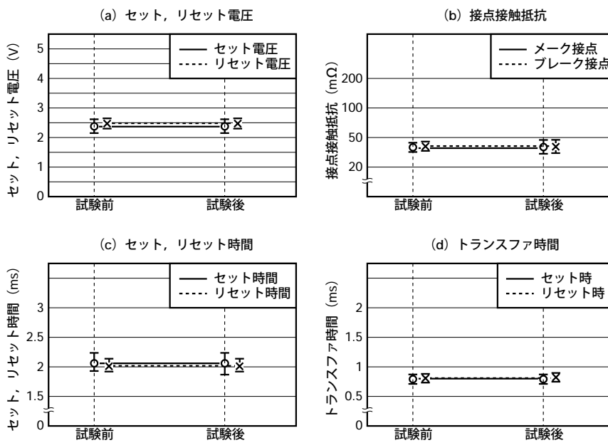
図5.6 (2) 衝撃
