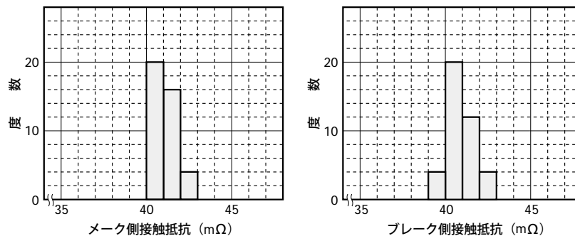
図4.5 接点接触抵抗
